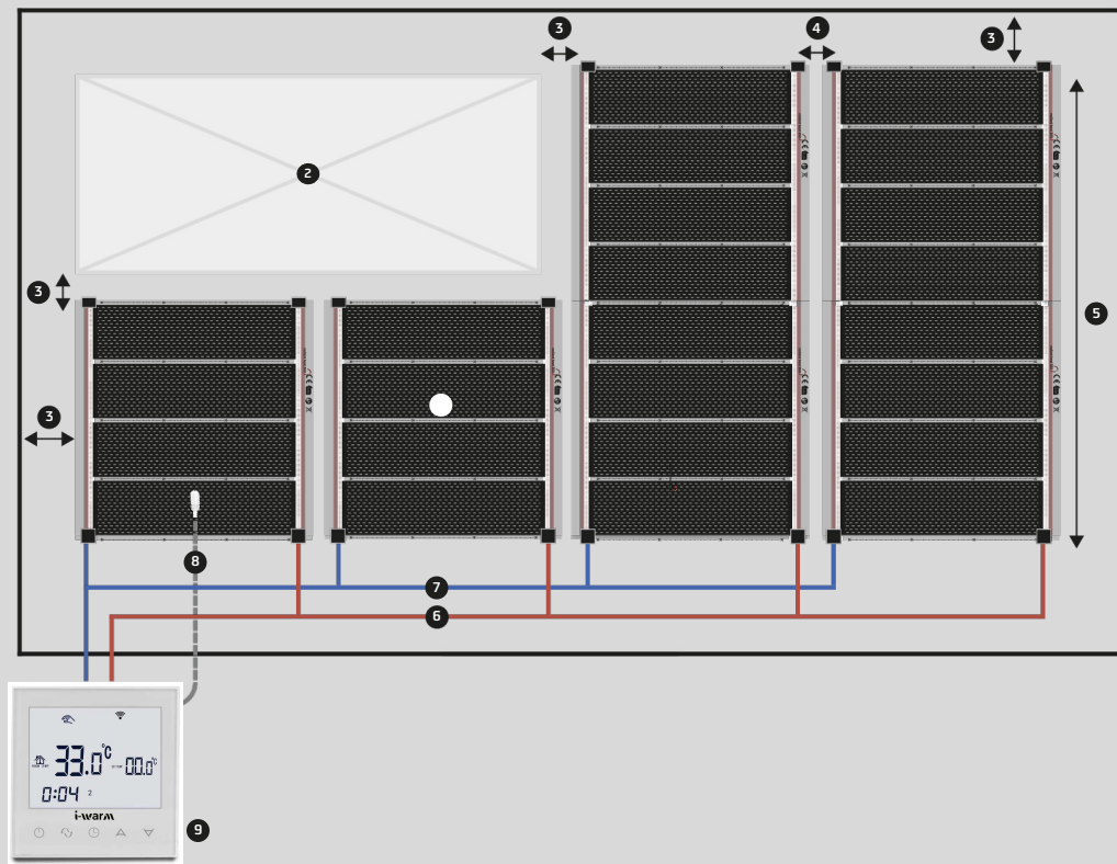
DIAGRAM 1: I-WARM FLUX HEATING FILM CONNECTION
